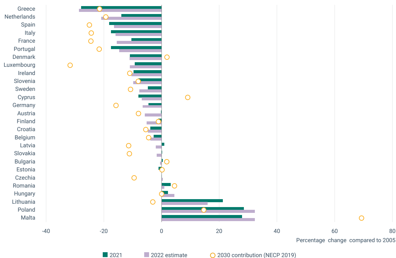
Figure 3.4 National progress towards 2030 Final energy consumption contributions
